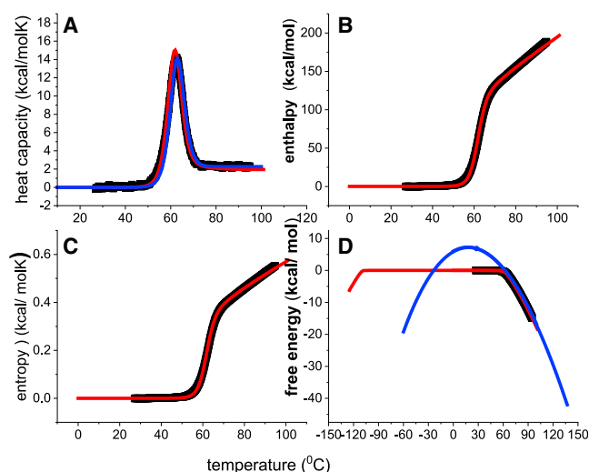
FIGURE 1 Differential scanning calorimetry of 50 \mu\text{M} lysozyme in 20\% glycine buffer, pH 2.5. Black data points: DSC thermograms obtained with a heating rate of 1^\circ\text{C min}^{-1} and a step size of 0.17^\circ\text{C} . Red lines: simulations with the Zimm-Bragg theory with h_0 = 1.0 kcal/mol, c_v = 6 cal/molK, \sigma = 1.0 \times 10^{-6} , \nu = 129 . (A) Heat capacity C_p(T) . (B) Unfolding enthalpy H(T) . (C) Unfolding entropy S(T) . (D) Free energy of unfolding G(T) . Blue line: \Delta G(T) (Eq. 13) predicted by the two-state model calculated with a conformational enthalpy \Delta H_0 = 107 kcal/mol and a heat capacity increase \Delta C_p^0 = 2.269 kcal/mol. Data taken from reference (10).
