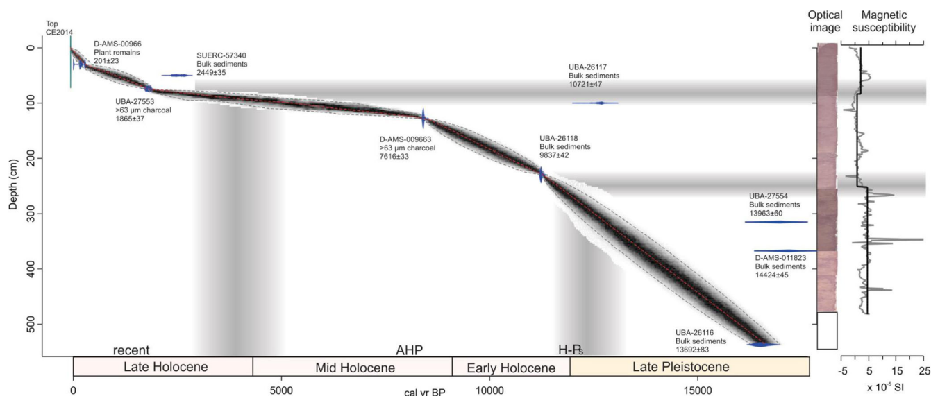
Figure 2. Age–depth model developed from nine radiocarbon dates using the Rbacon package (Blaauw and Christen, 2011) and weighted mean (red dashed line) and the 95% confidence interval of ~8 million random walks through the calibrated radiocarbon age probability densities (Reimer et al. , 2013) (low and upper limit = grey line). Optical image and magnetic susceptibility measured during ITRAX core scanning (see Methods). Down-core zonations were defined using the magnetic susceptibility, ITRAX and pollen assemblage zones, showing broad agreement in major changes in the sediment stratigraphy. Geological stages of the Quaternary (Walker et al. , 2019) are shown below. AHP, African Humid Period (Demenocal et al. , 2000); H, Holocene; Ps, Pleistocene. Note that there was no optical image or magnetic susceptibility data for the deepest section of core from 450–537 cm. [Color figure can be viewed at wileyonlinelibrary.com ]
