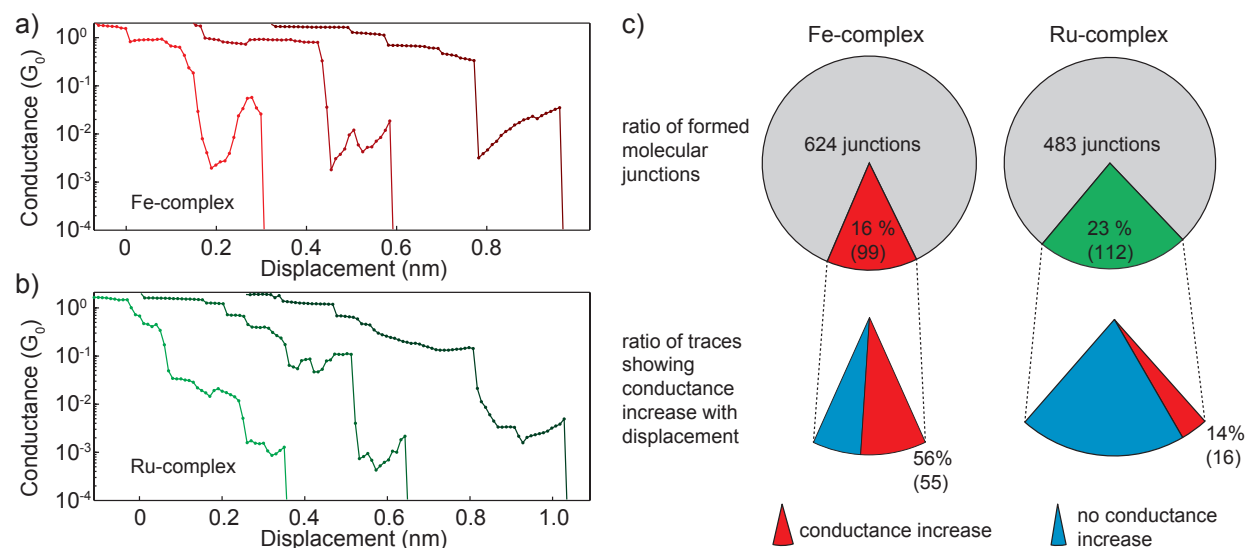
Figure 2: Conductance measurements. a-b) Three examples of conductance traces as a function of electrode displacement measured respectively in the presence of the \text{Fe}^{\text{II}} -complex and \text{Ru}^{\text{II}} -complex. c) Junction-formation statistics and percentage of molecular junctions showing a conductance increase.
