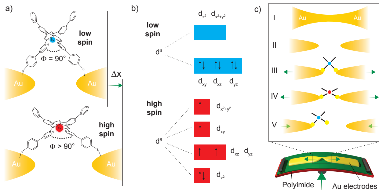
Figure 1: Two-terminal mechanically controlled single-molecule junction. a) Sketch of the Fe II -based SCO molecular junction in the ideal arrangement to trigger the LS to HS switch by separating the electrodes by \Delta x . b) Iron II 3d levels involved in the spin-crossover phenomenon. c) Schematic illustration of a mechanically controllable break junction (MCBJ) set-up (bottom) with the molecule placed in the junction as sketched in (a). A freely suspended gold bridge, built on a flexible substrate, is elongated upon bending the substrate in a mechanically controlled three-point bending mechanism. The predefined breaking point of the gold structure is enlarged on the top of the figure at different stages of the experiment: (I) elongation of the gold wire with the help of the pushing rod and two opposing counter supports (see bottom of the figure). (II) Rupture of the gold wire resulting in the formation of two gold nano-electrodes facing each other. (III) The metal complex may bridge both nano-electrodes and (IV) eventually one could manipulate the spatial arrangement of the complex's ligands by stretching of the junction. After the final rupture of the junction the electrodes can be moved toward each other (V) to start a new experiment.
