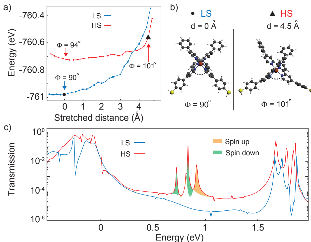
Figure 4: Theoretical calculations. a) Energy of the LS and HS states as a function of stretching distance found from DFT calculations. b) Relaxed geometries of the LS and HS states at the stretching distance of 0 Å and 4.5 Å respectively. c) Total transmission of the LS and HS geometries shown in (b) in a metal-molecule-metal configuration calculated with self-consistent DFT-NEGF. The shaded areas correspond to spin polarized transmission for up (orange) or down (green) spin electrons. The Fermi energy of the contacts is at 0 eV.
