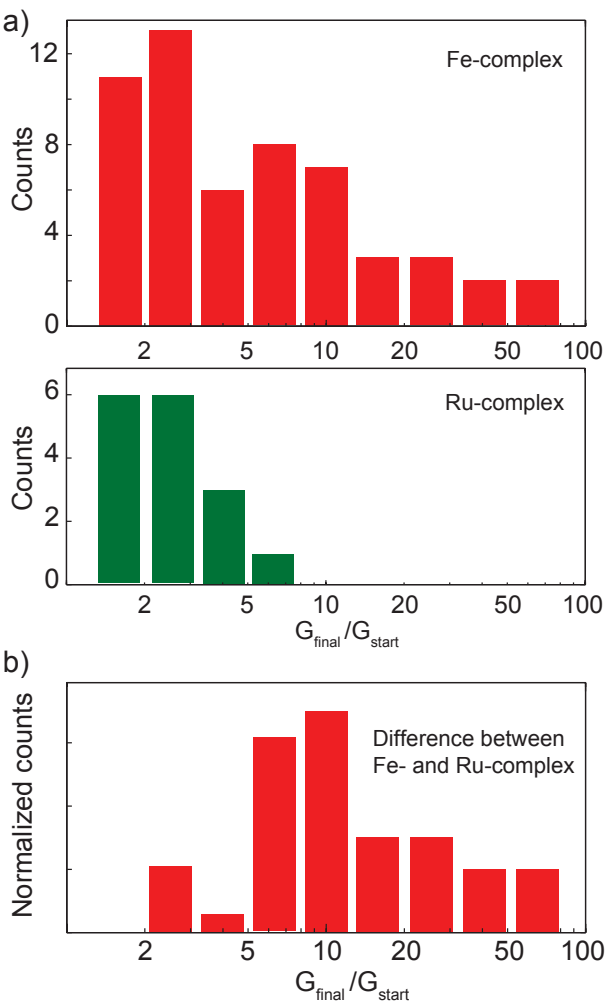
Figure 3: Statistics of conductance increase. a) Histogram of the values of increase in conductance for molecular junctions containing Fe (top) and Ru (bottom) complexes. The x-axis is binned logarithmically. b) Difference between the conductance ratio histograms of Fe II and Ru II after normalization (see supporting information).
