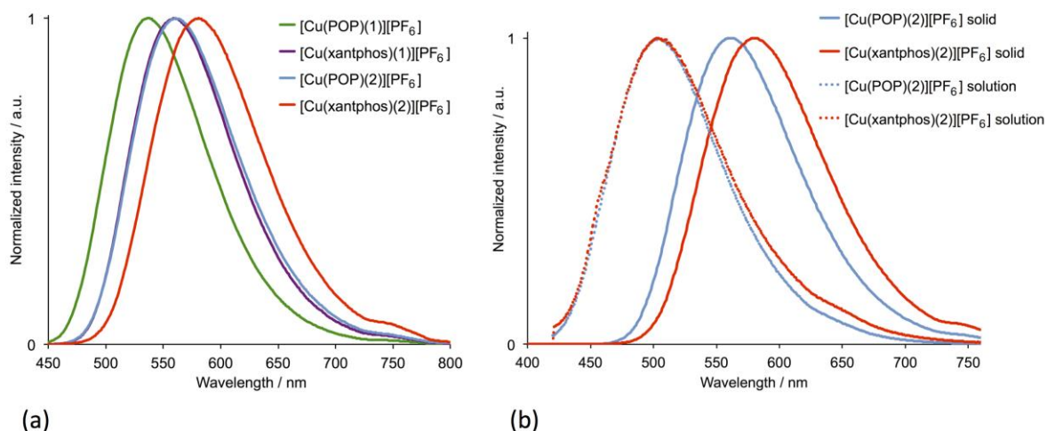
Figure 10. (a) Normalized emission spectra of powdered samples of the [\text{Cu}(\text{P}^{\wedge}\text{P})(\text{N}^{\wedge}\text{N})][\text{PF}_6] complexes ( \lambda_{\text{exc}} = 365 \text{ nm} ). (b) Normalized emission spectra of solution ( \text{CH}_2\text{Cl}_2 , 2.5 \times 10^{-6} \text{ mol dm}^{-3} ) and powdered samples of the [\text{Cu}(\text{P}^{\wedge}\text{P})(2)][\text{PF}_6] complexes ( \lambda_{\text{exc}} = 365 \text{ nm} ).
