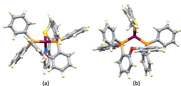
Fig. 4 Structures of (a) [\text{Cu}(\text{POP})(1)]^+ and (b) [\text{Cu}(\text{POP})(3)]^+ cations emphasizing the tetrahedral \text{Cu}(\text{I}) centre in the former and the sterogenic coordinated S-atoms.
