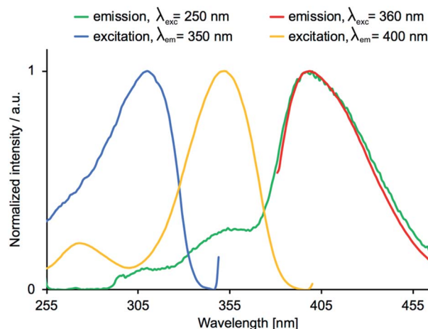
Fig. 12 Emission (red and green) and excitation (yellow and blue) spectra for a \text{CH}_2\text{Cl}_2 solution of [\text{Cu}(\text{POP})(2)][\text{PF}_6] .
