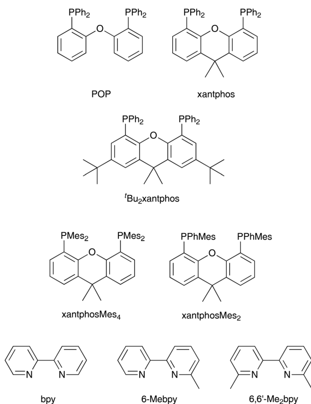
Scheme 1 Structures of the P^P and N^N ligands.
