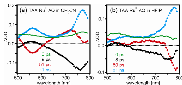
Figure 5. (a) Decay component spectra and calculated time-resolved spectrum at 0 ps obtained from global fits of decay curves measured after excitation of the ruthenium(II) triad at 420 nm in \text{CH}_3\text{CN} with femtosecond laser pulses (see Experimental Section for details). (b) Analogous data obtained for the ruthenium(II) triad in HFIP.
