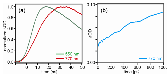
Figure 6. (a) Rise of the transient absorption signals at 550 nm (green trace) and 770 nm (red trace) after excitation of the TAA-Os II -AQ triad at 532 nm with laser pulses of ~8 ns width (CH 3 CN solution). (b) Rise of the transient absorption signal at 770 nm after exciting the same triad at 420 nm with laser pulses of ~200 fs duration (HFIP solution).
