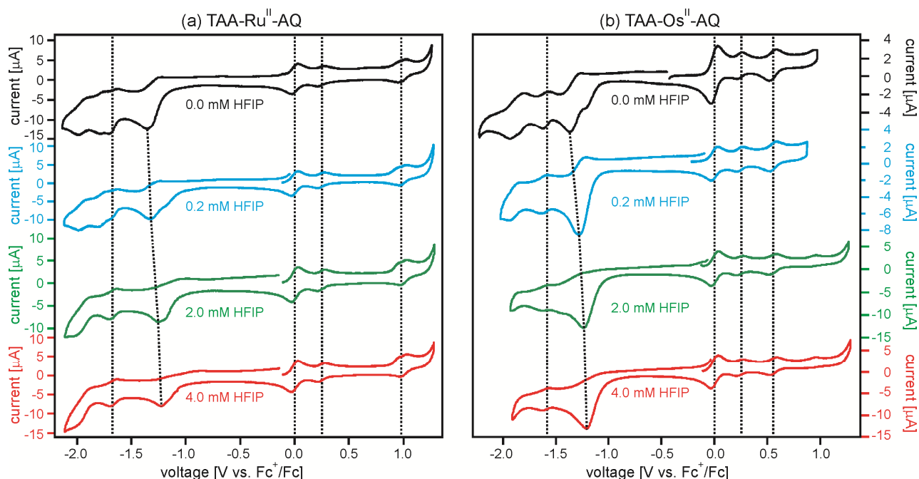
Figure 8. Cyclic voltammograms obtained from TAA-Ru II -AQ (a) and TAA-Os II -AQ (b) in dry and deoxygenated \text{CH}_2\text{Cl}_2 in presence of increasing concentrations of hexafluoroisopropanol (from top to bottom). The supporting electrolyte was 0.1 M TBAPF 6 , the waves at 0.0 V vs. \text{Fc}^+/\text{Fc} are due to the ferrocene reference.
