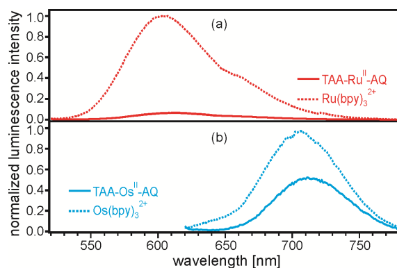
Figure 2. Luminescence spectra of the two triads from Scheme 1 in aerated \text{CH}_3\text{CN} compared to those of \text{Ru}(\text{bpy})_3^{2+} and \text{Os}(\text{bpy})_3^{2+} measured under identical conditions. Excitation occurred at 450 nm in all cases, the intensities are normalized to a value of 1 at the band maxima of the reference complexes; differences in absorbance at the excitation wavelength were taken into account when normalizing.
