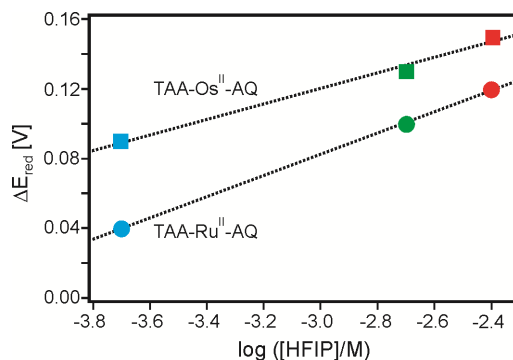
Figure 9. Shifts of the \text{AQ}/\text{AQ}^- reduction potentials ( \Delta E_{\text{red}} ) in \text{TAA-Ru}^{\text{II}}\text{-AQ} (circles) and \text{TAA-Os}^{\text{II}}\text{-AQ} (squares) as a function of HFIP concentration in \text{CH}_2\text{Cl}_2 . The color code corresponds to that used in Figure 8. The dotted straight lines are linear regression fits used for the determination of K_{\text{eq}} (eq. 2).
