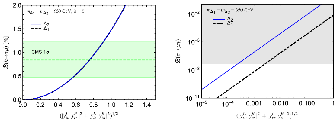
Figure 7. (Left-hand side panel) Higgs branching ratio to \tau\mu final state in the presence of scalar leptoquarks \Delta_1 = (\mathbf{3}, \mathbf{1}, -\mathbf{1}/\mathbf{3}) and \Delta_2 = (\mathbf{3}, \mathbf{2}, \mathbf{7}/\mathbf{6}) with Higgs portal coupling \lambda set to zero. (Right-hand side panel) \tau \rightarrow \mu\gamma constraints. The \Delta_1 ( \Delta_2 ) case is rendered in dashed (solid) line. The following transformation needs to be applied when going from the \Delta_1 to the \Delta_2 case: y_{ij}^L \rightarrow y_{ji}^L .
