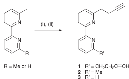
Scheme 4 Syntheses of compounds 1–3 . Conditions: (i) LDA, THF, -78\text{ }^\circ\text{C} ; (ii) propargyl bromide (1.8 molar equivalents for 1 , 0.8 equivalents for 2 and 3 ), THF, -78\text{ }^\circ\text{C} warm to 22\text{ }^\circ\text{C} , ca. 15 h.
