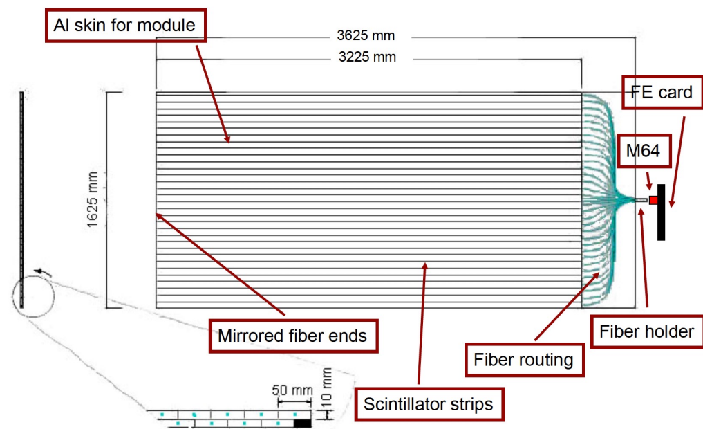
Figure 49. Labeled illustration of a CRT module.
