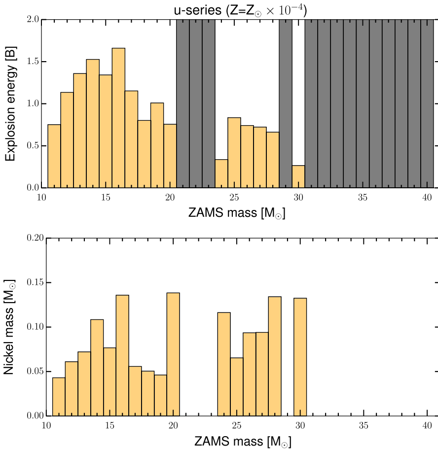
Fig. 21 Results of core-collapse supernova simulations for stars with a low metallicity ( [\text{Fe}/\text{H}] = -4 ) as a function of progenitor mass. Typical explosion energies of 1 Bethe ( = 10^{51} erg) are found up to about 30 M_{\odot} . For higher masses, the collapse leads to black hole formation. There exists also a narrow mass range between 20 and 30 M_{\odot} where black hole formation takes place, due to the structure/compactness of these specific stellar models. Explosions occur typically 300 to 700 ms after collapse. The amount of ^{56}\text{Ni} ejecta ranges from about 0.04 to 0.12 M_{\odot} (for SN1987A 0.07 M_{\odot} was determined observationally). Similar results are found in Ertl et al. (2016). Image reproduced with permission from Ebinger et al. (2020), copyright by AAS
