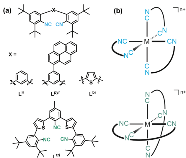
Fig. 2 (a) Molecular structures of the chelating diisocyanide ligands L^H , L^{Pyr} , L^{bi} and the trisocyanide ligand L^{tri} . (b) Generic structures of homoleptic tris(diisocyanide) (up) and bis(triisocyanide) (down) complexes. M = \text{Cr}^0 , n = 0 ; M = \text{Mn}^I , n = 1 .
