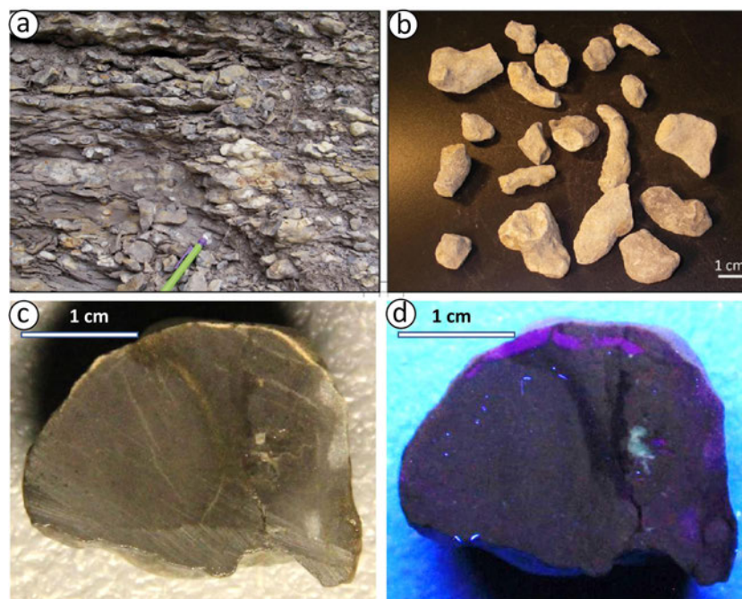
Figure 5. Facies 2 (F2): nodular marl. (a) Outcrop view. (b) Individual nodules and nodule clusters. (c, d) Cross section of a nodule under natural (c) and UV light (d); the vertical parting in the middle of the sample that shows a darker color in (c) but is non-fluorescent in (d) is suggestive of previous boundary between two, now clustered nodules.
