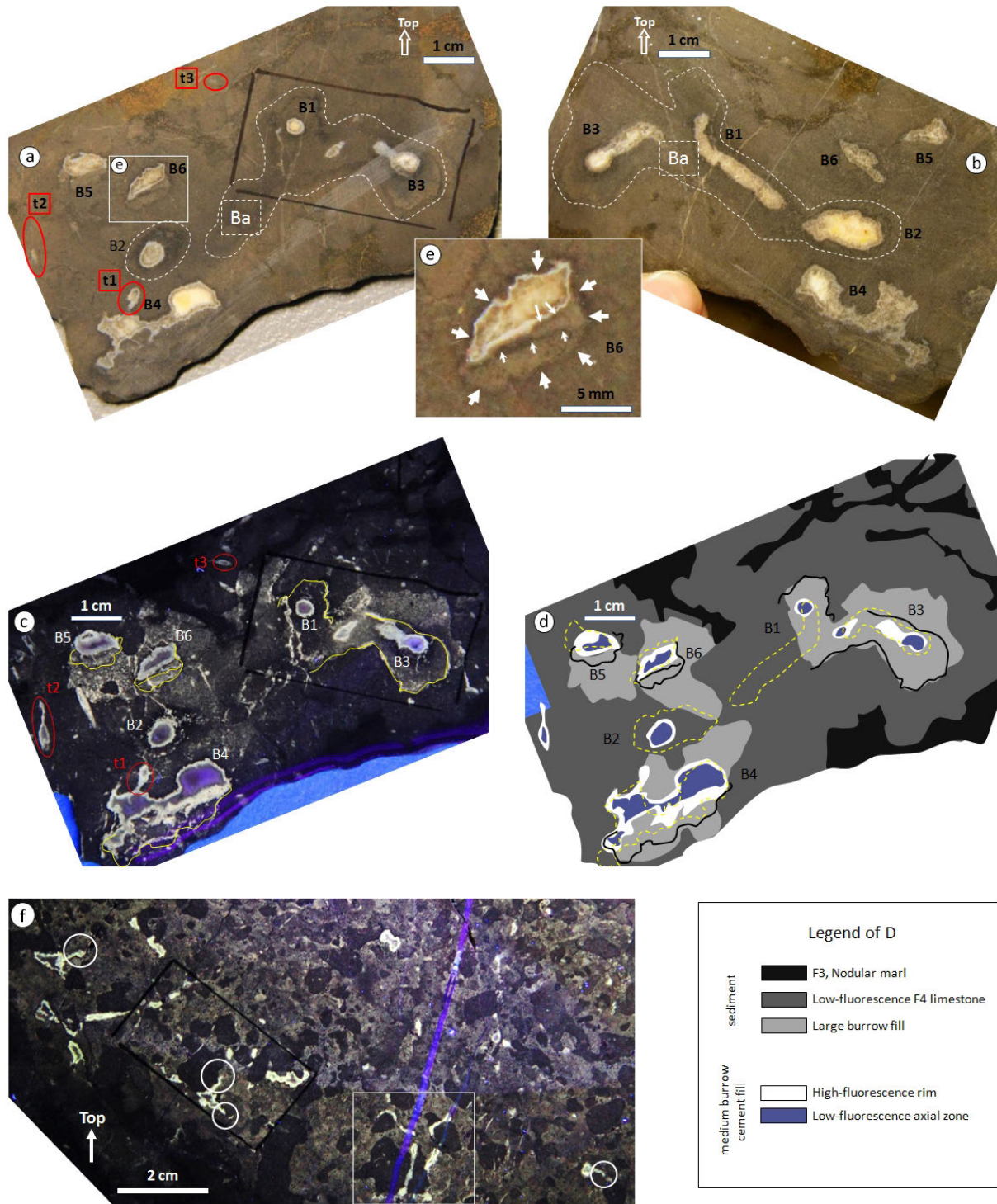
Figure 9. Burrow architecture in F4. (a, b) Opposing sides of a saw cut, ca. 3 mm apart; Note three types of burrows: large burrows (one marked as Ba) surrounded by white dashed line; medium burrows (partly) filled with white-yellowish cement (labeled B1–B6); small burrows (t1–t3) encircled in red. The white rectangle in (a) is the position the close-up shown in panel (e). (c) UV-light view of the section shown in (a). Yellow lines follow main dark halos, as marked in (a). (d) Line drawing of (c); black lines are dark halos copied from (c), yellow dotted lines are the position of dark halos on the opposite side of the saw cut (drawn on b and flipped), illustrating changes in burrow size and orientation across the 3 mm gap between the sections. (e) Close-up of B6 marked in (a) showing burrow surrounded by dark halo (bold arrows) and half-filled with geopetal sediment; thin white arrows show halos inside the geopetal filling. (f) Cross-cutting relationships between burrows (UV fluorescence). White circles point at small burrows connected to adjacent medium burrows. The white rectangle highlights longitudinal cross sections of small burrows. Black rectangles were drawn during the sample preparation process for thin section selection
