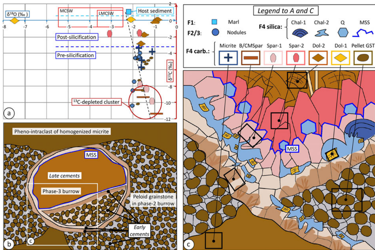
Figure 13. Stable C and O isotopes and microfacies. (a) Sedimentary and diagenetic carbonate phases encountered in the Aurel pseudobioherm in \delta^{13}\text{C} – \delta^{18}\text{O} plot; the position of samples of facies F1 to F3 is shown in Fig. 14. MCSW: middle-Callovian seawater composition; LMCSW: subset for the lower part of the middle Callovian (Pellenard et al., 2014). (b) Fabric and microfacies of F4 recording successive phases of bioturbation; the white box indicates the general position of (c) . (c) Schematic geometric relationships between sediment and various cement generations within Facies F4; black boxes mark minimum size of samples drilled for isotope analysis, some likely mixing different phases like peloid grainstone and BMSpar/CMSpar. GST: grainstone. Chal-1: early botryoidal chalcedony; Chal-2: later replacement chalcedony; Q: euhedral quartz crystals; MSS: main silicification surface; BMSpar and CMSpar: brown and clear microsparite, respectively; Spar-1: pre-silicification sparite; Spar-2: post-silicification sparite; Dol-1: syn-silicification saddle dolomite; Dol-2: late saddle dolomite; GST: grainstone. For details, see the text.
