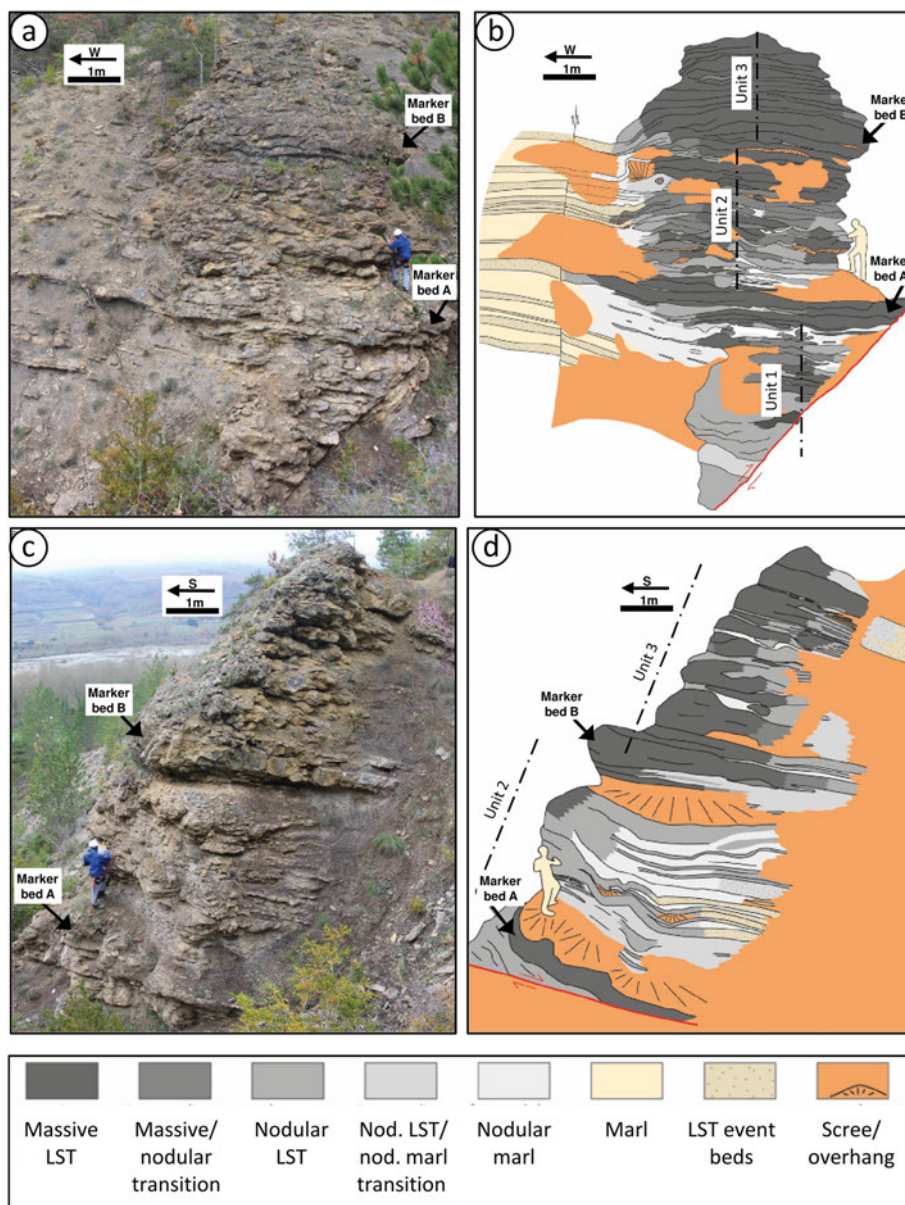
Figure 3. (a, b) Image and interpretation of the southern flank of the Aurel pseudobioherm; dashed lines represent assumed axis of the pseudobioherm. (c, d) Image and interpretation of the eastern flank of the pseudobioherm. LST: limestone.
