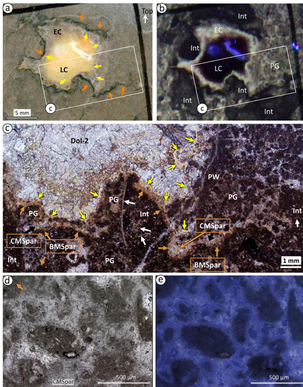
Figure 10. (a, b) Close-up of Fig. 8a and b showing the details of burrow infill; white rectangle marks the position of the thin section close-up in (c). (a) Natural light view; EC: early cements, LC: late cements; the orange arrows mark a dark halo surrounding the burrow on the left side and opening into sediment on the right side; yellow arrows mark a thin, continuous, milky white cement rim following the dark halo on the left side of the image but following the sediment-cement contact on the right side. (b) UV fluorescence view indicates that the fluorescent halo expands on the right side into peloid grainstone (PG); the blurry appearance results from the diffusion of light emitted from fluorescent parts into non-fluorescent ones; Int: micrite pheno-intraclasts; pheno-intraclasts, like nodules in F2 and F3 exhibit a low level of fluorescence. The brightly fluorescent zone is bounded by the dark rim on the outer side (orange arrows in a) and the white rim on the inner side of the burrow (yellow arrows in a). (c) Microphotograph of the sample shown in (a) and (b) (plane-polarized light view); the dark halo (orange arrows) corresponds to the superposition of brown and clear microsparite layers (BMSpar and CMSpar, respectively), with BMSpar directly covering the burrow wall. The white rim (yellow arrows) consists of beige chalcidony (for details, see Fig. 11). The white arrows point to shell fragments, PW: peloid wackestone, Dol-2: late saddle dolomite. (d, e) Photomicrographs of peloid grainstone in F4. (d) Internal texture of the peloids in plane-polarized light; (e) As (d) in UV epifluorescent light.
