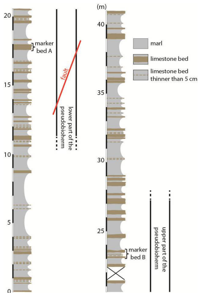
Figure 2. Lithologic log of the middle-Callovian deposits in the pseudobioherm-bearing interval, logged about 20 m to the west of the upper part of the pseudobioherm, not affected by faulting; note marker beds A and B, which are easily recognizable in both host sediment and pseudobioherm.
