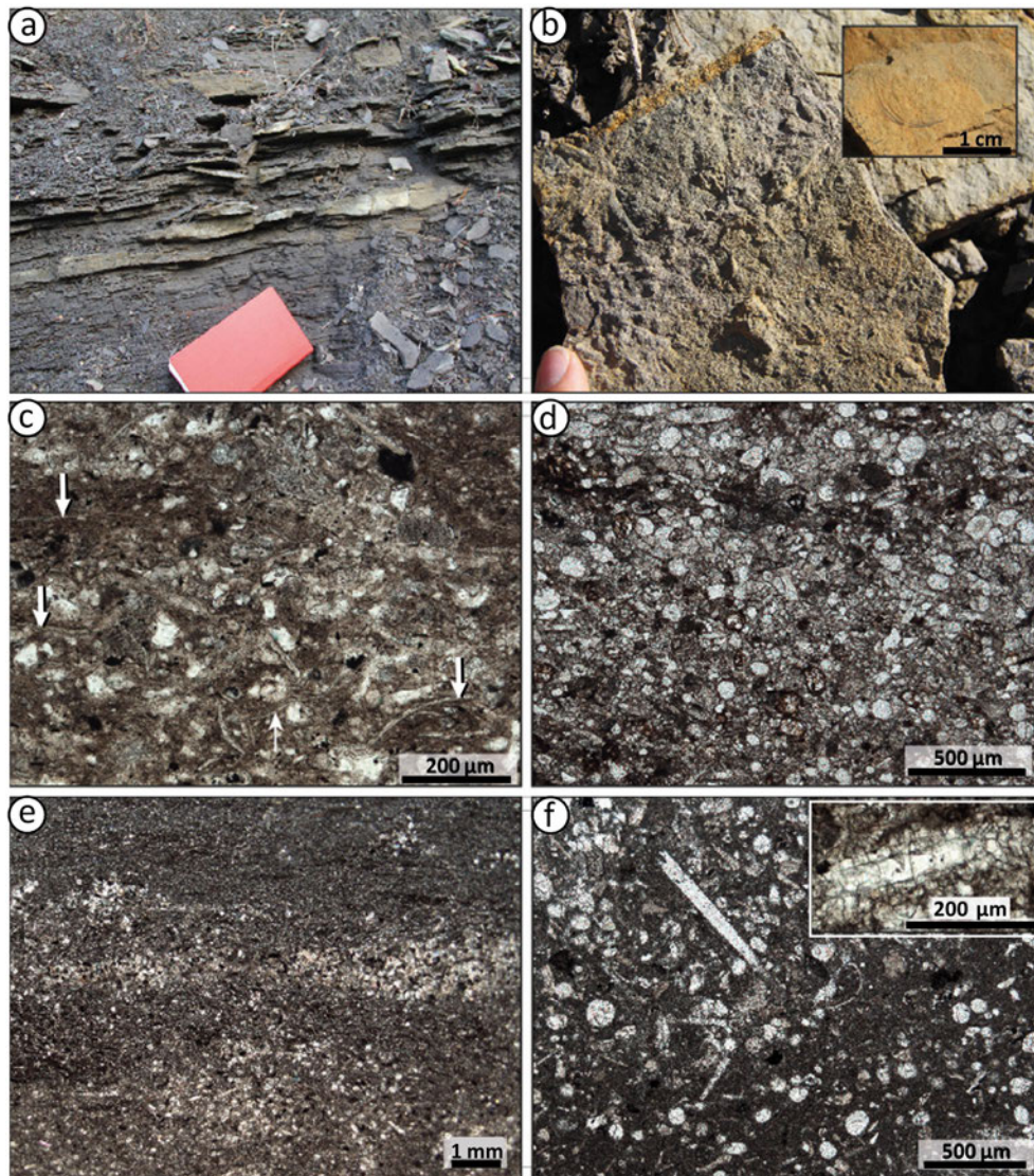
Figure 4. Background Facies 1 (F1). (a) Typical alternation between marl and limestone showing platy bedding. (b) Basal surface of a limestone slab with radiating burrow ( Gyrophyllites multiradiatus ); the inset shows the bivalve Bositra , the only common fossil in F1. (c) Marl with numerous filamentous structures (white arrows) interpreted as disaggregated Bositra shells. (d) Limestone showing the same microfossil content as the marl but in microsparitic matrix. (e) Limestone consisting of alternating packstone and wackestone laminae. (f) Marl with numerous recrystallized microfossils in a micritic matrix; circular objects are interpreted as calcispheres or radiolarians; the inset shows a tubular structure interpreted as a sponge spicule.
