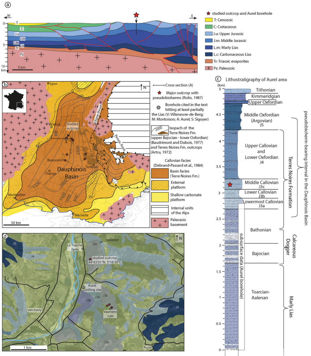
Figure 1. Geological setting of the studied outcrop. (a) Cross section from the margin to the center of the Dauphinois Basin traversing the Aurel borehole (modified after Wannesson and Bessereau, 1999). (b) Facies map of the Dauphinois Basin for the Callovian (Debrand-Passard et al., 1984). Isopachs (in m), after Baudrimont and Dubois (1977), are shown for the basin facies represented by the Terre Noires Formation (middle Bathonian up to lower Oxfordian) in the central part of the basin. Outcrops of the Terre Noires Formation (after Artru, 1972) are noted by a darker shade of brown, and the locations of major pseudobioherms are marked by red stars (after Rolin, 1987). (c) Lithologic log of the Aurel area (Flandrin, 1974). The Aurel borehole penetrated the carbonate-dominated Dogger and the marly upper Lias. The pseudobioherms in the Aurel area are hosted in middle-Callovian sediments (red star on the log); in the Dauphinois Basin, they generally occur in upper-Bathonian to middle-Oxfordian deposits. (d) Geological map of the Aurel area (modified after Flandrin, 1974). Several pseudobioherms are poorly exposed near the Vaunière ruin; the studied pseudobioherm is located near La Touche farm.
