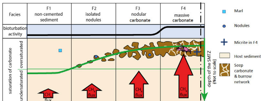
Figure 14. Change in depth of the sulfate–methane transition zone (SMTZ) and seep carbonates (brown) from host sediment towards the pseudobioherm; the vertical dashed line marks the axis of the pseudobioherm; geometric symbols refer to the isotope data shown in Fig. 13a; the decapod crustacean symbolizes the burrowers responsible for the gas-focusing burrow network. (Not to scale.)
