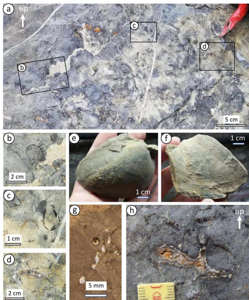
Figure 7. Facies 4 (F4): massive limestone and associated fauna. (a) Weathered surface showing three bivalves shown in (b) to (d) in detail, apparently belonging to different species. (d) Bivalve with geopetal filling. (e, f) Two valves of the only lucinid found (likely Beauvoisina carinata ; Kiel et al., 2010). (g) Section of a small gastropod. (h) Bedding plane view of Thalassinoides (smaller graduations on the tape measure are 1 mm apart).
