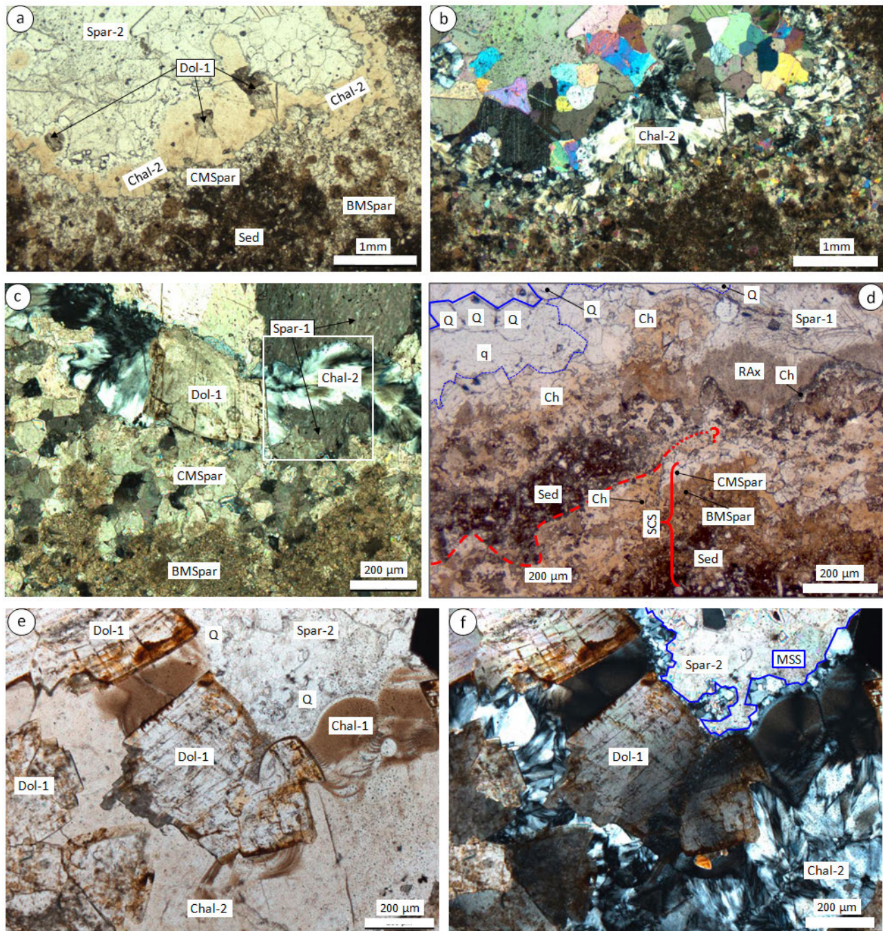
Figure 11. Cements within Phase-3 burrows and host sediment. (a, b) General view of burrow margin in plane-polarized light (a) and cross-polarized light (b) . Note continuous rim of beige chalcedony (Chal-2) associated with saddle dolomite (Dol-1); BMSpar and CMSpar: brown and clear microspar, respectively; Sed: sediment. (c) Details of the relationship between Chal-2 and carbonate cements in cross-polarized light; Spar-1: first generation of sparite cement; the white rectangle: Chal 2 cutting across a single sparite crystal. (d) Burrow rim in plane-polarized light showing one sediment–cement sequence (SCS, red bracket) capped by sediment in the left part. The cements are heavily replaced by chalcedony. Red line: top of SCS, dashed where observed and dotted where inferred. Radial gray calcite crystals (RAx) locally cap the SCS. Blue lines (dashed at base, solid at top) outline a patch of quartz with anhedral (q) capped by euhedral (Q) crystals; euhedral crystals are aligned roughly parallel to burrow margin wall. (e, f) Main phases of silicification in plane-polarized light (e) and cross-polarized light (f) ; Chal-1: botryoidal chalcedony precipitated freely at the tube wall, Q: euhedral quartz also overgrown on a free surface, Chal-2 and the associated saddle dolomite Dol-1 replaced both preexisting carbonates and Chal-1. Note the extinction pattern of Chal-2 characterizing “flamboyant chalcedony”. The blue zigzag line marks the main silicification surface (MSS). For details, see the text.
