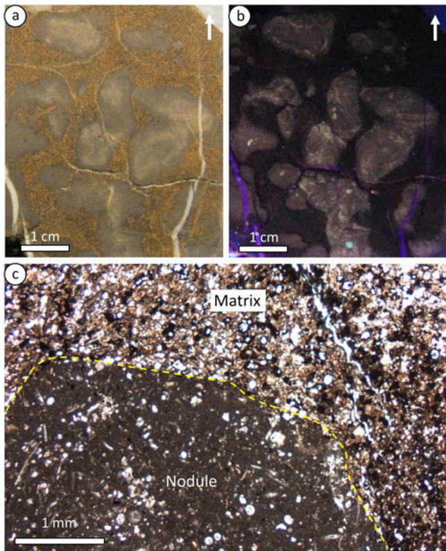
Figure 6. Facies 3 (F3): nodular limestone. (a, b) Vertical section under natural (a) and UV light (b); arrows point upward. (c) Photomicrograph showing contact between a nodule and matrix (marked by yellow dashed line). Grain packing in the matrix is denser than in the nodule, suggesting cementation of the nodule prior to compaction.
