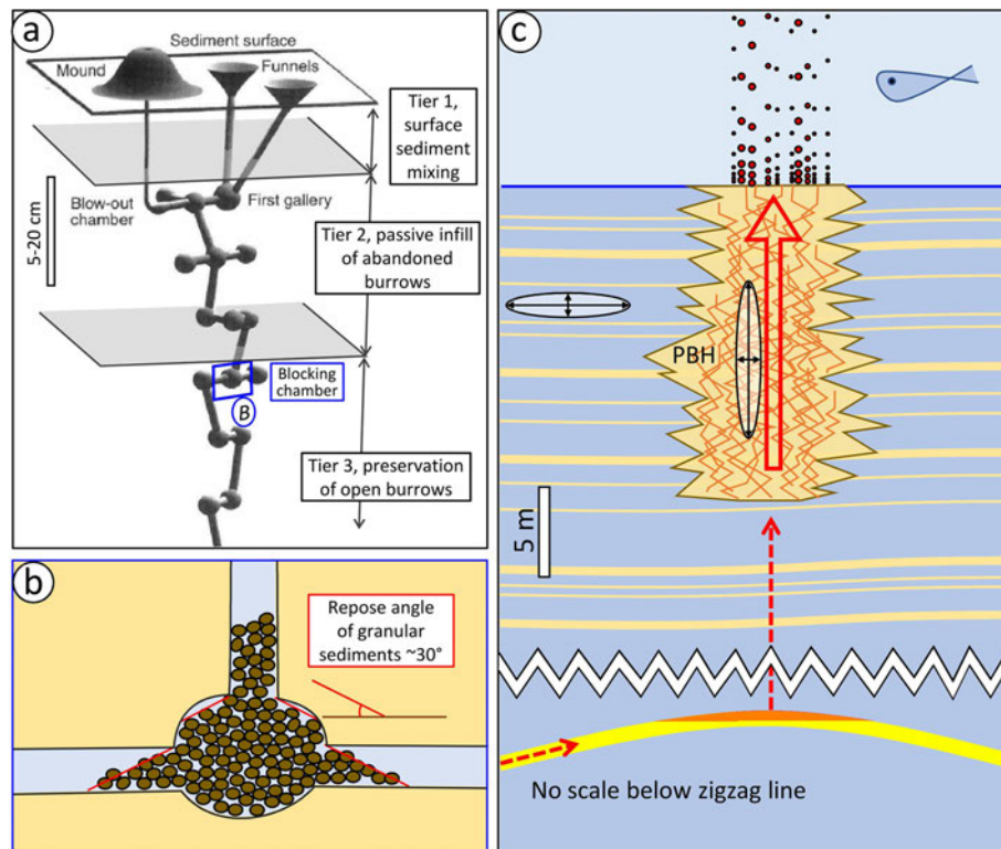
Figure 15. Fluid flow in and around the pseudobioherm (PBH). (a) Typical architecture of a recent decapod crustacean burrow ( Callinassa truncata , modified after Ziebis et al., 1996); gray surfaces indicate the hypothetical limits between bioturbation tiers 1 and 3 in Aurel (tier 4 below shown interval). The blue frame marks the shallowest chamber acting as trap for sediment shed from above and minimizing further downward sediment transfer. (b) Close-up of trapping chamber; once lateral spill-out from the chamber reaches angle of repose (ca. 30^\circ , Allen, 1992), additional sediment from above piles up in the shaft and deeper parts of the burrow remain open. (c) Sketch of fluid circulation in and around the Aurel pseudobioherm (PBH) during its formation. The lower part represents the hypothetical deep structure focusing late thermogenic methane into the pseudobioherm; red dashed arrows at depth indicate hypothetical gas migration pathways from a source rock into the structure and further up to the base of the pseudobioherm. The upper part shows the circulation pattern of gas and compaction fluids within the pseudobioherm; orange zigzag lines represent crustacean burrows providing a connected tube network down to the bottom of the pseudobioherm. White ellipses represent permeability tensors in the pseudobioherm and host sediment, with the principal axes of minimum and maximum permeability shown by black arrows; red arrow within the pseudobioherm marks the vertical flow pattern of the gas (-charged fluids), likely with episodic escape of gas at the seafloor (red bubbles in the water column).
