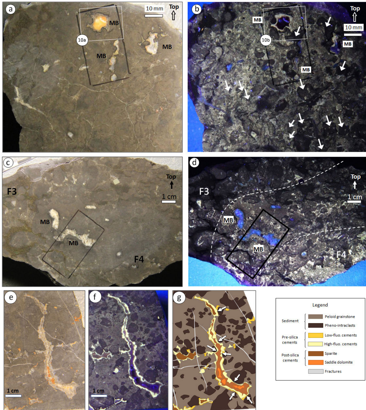
Figure 8. Fabric of intensely bioturbated sediment. (a) Natural light and (b) UV fluorescent light, Facies F4. White arrows in (b) point at some of the micrite pheno-intraclasts. Note the variability of pheno-intraclasts in roundness and size. MB: medium burrow. (c) Natural light and (d) UV fluorescent light, transition from F3 to F4. In both samples, MBs appear independent of variations in the fabric around them; black rectangles were drawn for thin section selection. (e) Natural light, (f) UV fluorescent light and (g) line drawing, Facies F4, unoriented vertical section. White arrows in (g) show points where the burrow's edge is tangent to pheno-intraclasts.
