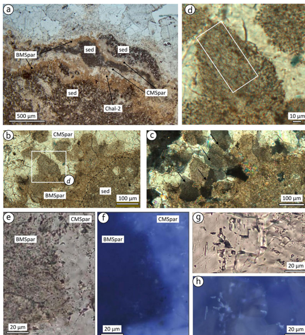
Figure 12. Microphotographs showing details of sediment–cement sequences. (a) Repeated sequence of sediment (sed), brown microsparite (BMSpar), and clear microsparite (CMSpar), locally overprinted by chalcedony (Chal-2). (b) Detail of BMSpar–CMSpar contact (black dashed line follows the underlying BMSpar–sediment contact); BMSpar appears as a set of filamentous “bushes”; the white rectangle marks the area shown in detail in (d) . (c) As (b) in cross-polarized light, showing individual microspar crystals straddling across BMSpar–CMSpar boundaries (marked by black arrows). (d) Close-up of filamentous bush; note the elongate brown inclusions within clear crystal, particularly in white rectangle. (e, f) BMSpar–CMSpar contact in plane light (e) and UV epifluorescent light (f) ; fluorescent inclusions near the margin of BMSpar following oblique contact between BMSpar and CMSpar into the thin section. (g, h) Typical CMSpar in plane light (g) and UV epifluorescent light (h) , fluorescence originating from both fluid inclusions (bright white) and microspar (dull yellow).
