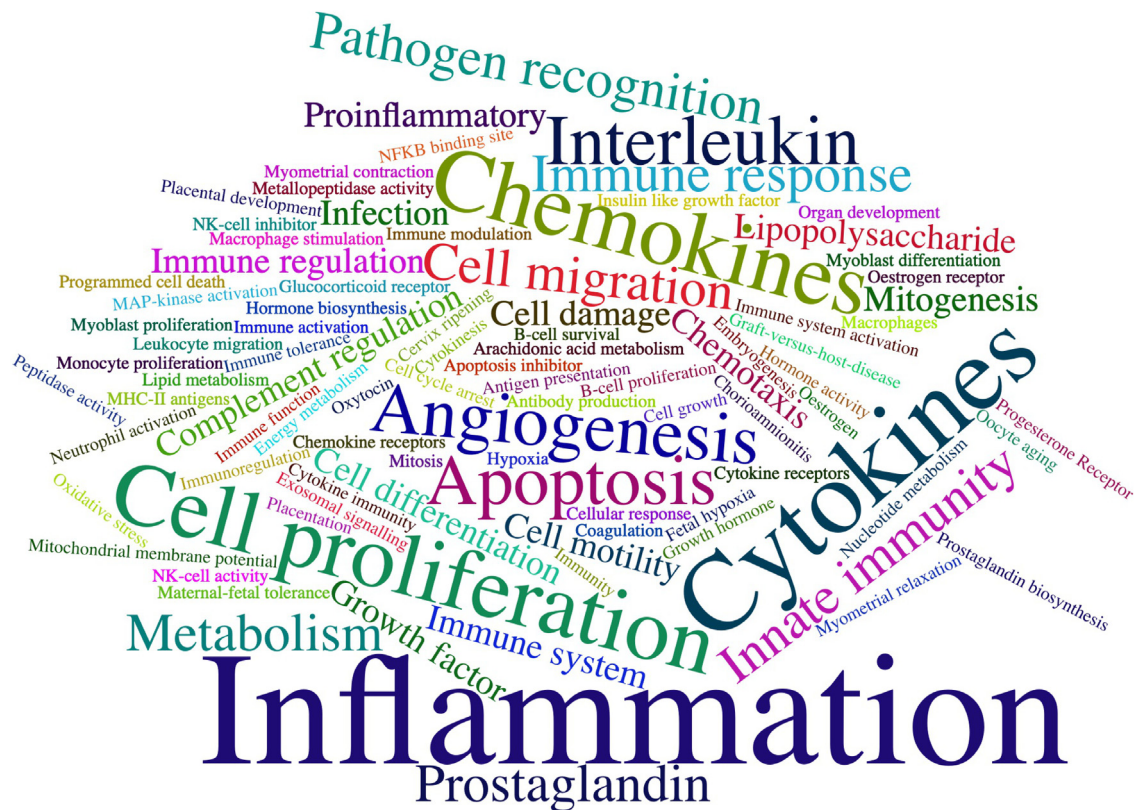
Fig. 2. Keywords of most commonly encountered gene functions and associated biological pathways. Font size is proportional to the number of times the words were encountered.
