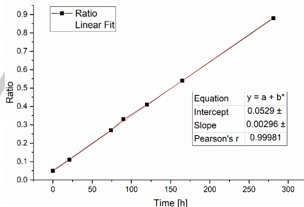
Figure 1. Ratio of unsymmetrical p -methoxyphenyl p -methylphenyl disulfide to symmetrical p -methoxyphenyl disulfide.
