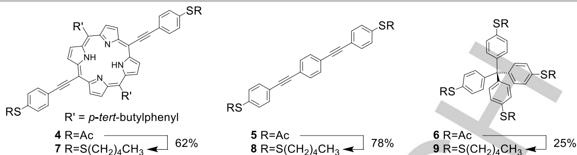
Scheme 3. Example of relevant molecules bearing multiple asymmetric disulfides synthesized from the corresponding thioacetates and S -pentyl benzene thiosulfonate using the here reported one-pot method. The displayed yields are the isolated amounts after column chromatography.
