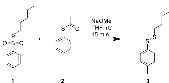
Scheme 1. Proof-of-concept reaction using 1 (1.10 eq.), 2 (1.00 eq.) and sodium methoxide (1.20 eq.) in THF at room temperature.
