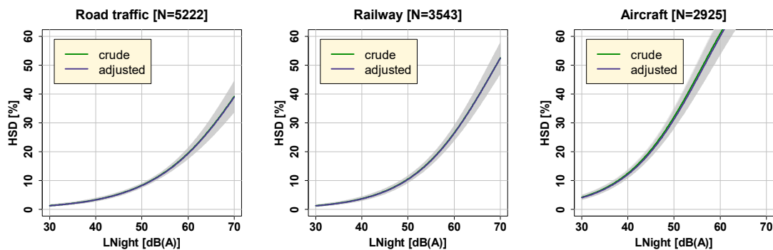
Figure 3. %HSD as function of LNight at the maximum façade point for road traffic, railway, and aircraft noise. The curves reflect both the crude and adjusted model with covariates centered on the mean (i.e., for the road traffic model: male sex = 0.47; age = 49; German language = 0.66; interview mode postal = 0.78 – for the railway model: male sex = 0.49; age = 48; German language = 0.69; interview mode postal = 0.77 – for the aircraft model: male sex = 0.47; age = 48; German language = 0.74; interview mode postal = 0.76.). The curves include 95% (overlapping) confidence intervals as shaded areas.
