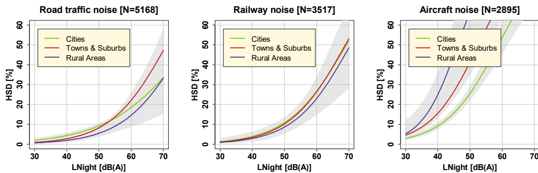
Figure 7. Exposure-response relationships for road traffic (left), railway (middle), and aircraft noise (right), for different degrees of urbanization in the municipality of the respondent’s dwelling unit, including 95% (partly overlapping) confidence intervals (shaded areas). Curves are based on the adjusted model in the full sample with covariates centered on the mean.
