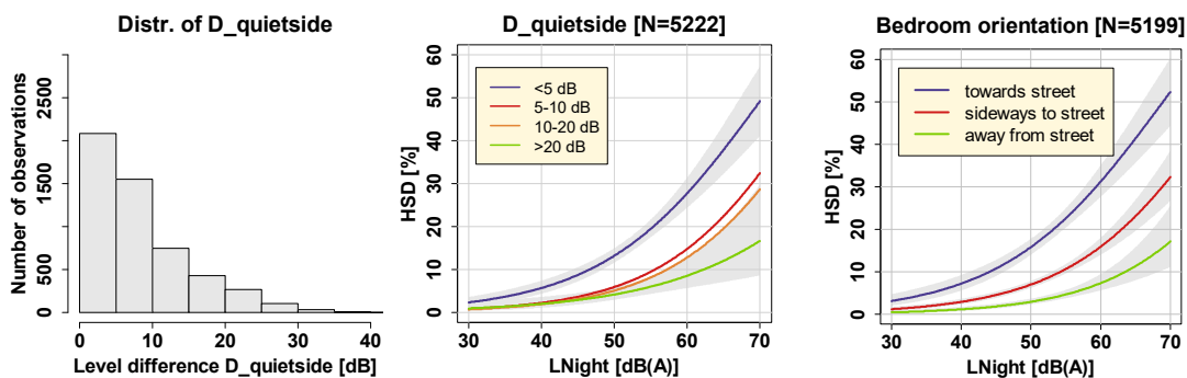
Figure 6. Left: Frequency distribution of the level difference indicator D_quietside. Middle: Exposure-response relationships for road traffic noise for four groups of D_quietside; 95% confidence intervals as shaded areas shown for the <5 dB and >20 dB category only. Right: Exposure-response relationships for road traffic noise for different orientations of the bedroom window, including 95% confidence intervals as shaded areas. LNight always refers to the maximum façade point of the dwelling unit. Curves are based on the adjusted model in the full sample with covariates centered on the mean.
