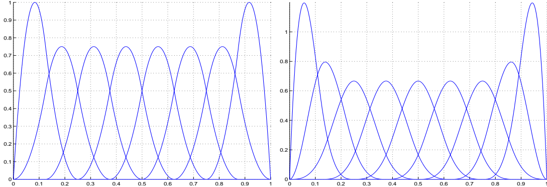
Figure 1: Quadratic (left) and cubic (right) B-splines on level j = 3 on the interval [0, 1] .
