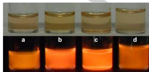
Figure 7. Photographs of 0.5 \mu\text{M} CdSe-5ZnS QDs (entry 7 in Table 1) capped with DHLA-TBA + in methanol (a), acetonitrile (b), DMSO (c) and water (d) under ambient light (top) and UV light (365 nm, bottom). Adapted by permission of the Royal Society of Chemistry. [26a]
