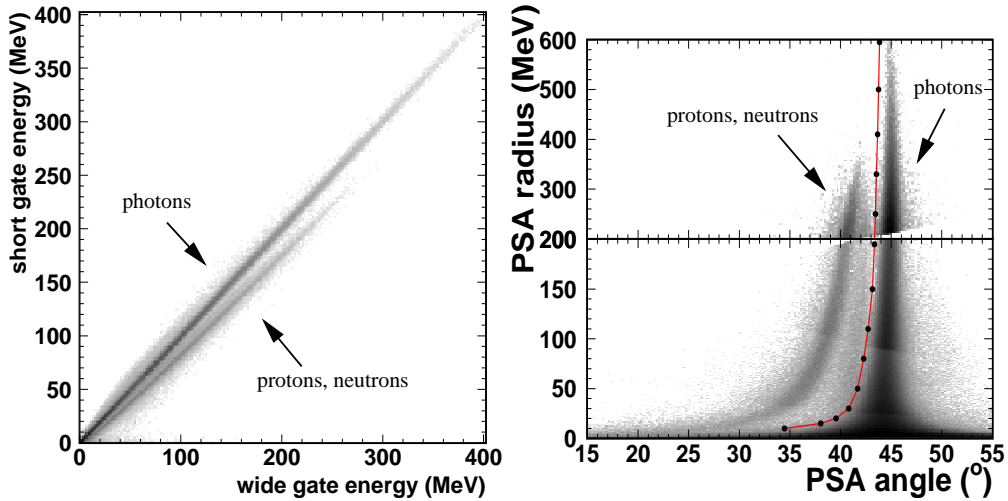
Figure 3.3: Typical pulshape plot for a BaF 2 detector of the forward wall. Left: E_{wide} (full energy) is plotted vs E_{short} (only the fast component). The photons lie on a line E_{wide} = E_{short} . Right: same plot using polar coordinate (explained in text). Photons are chosen as being to the right of the line. Both representations use a logarithmic scale as most detected particles are photons.
