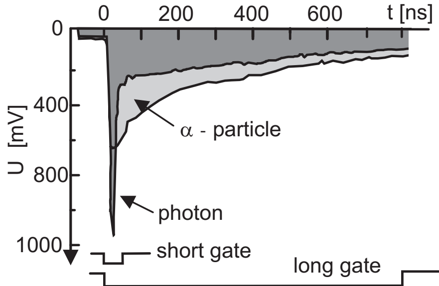
Figure 2.5: typical pulse shape representation for an alpha particle and a photon signal in the BaF 2
