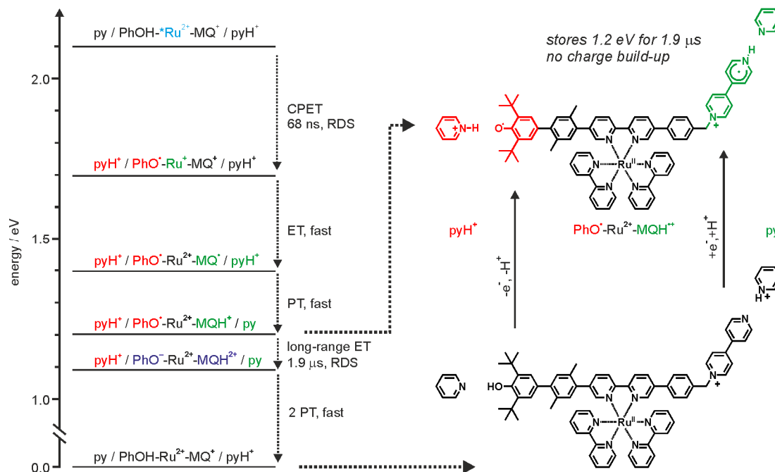
Scheme 1. Energy level scheme illustrating the key elementary steps leading to the formation of the long-lived PhO • / MQH •+ radical pair and its subsequent decay (see SI pages S21-S32 for details). CPET = concerted proton-electron transfer, ET = electron transfer, PT = proton transfer, RDS = rate determining step.
