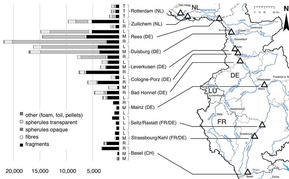
Figure 1. Number of microplastic particles ( 300\ \mu\text{m} - 5\ \text{mm} ) 1000\ \text{m}^{-3} in categories at all sampling sites ( \Delta ). The horizontal columns present microplastic abundance 1000\ \text{m}^{-3} and the respective fraction of categories. L: left bank, M: mid-river, R: right bank, T: transect (position in the river cross section). The figure was created using Adobe Photoshop CS4, Version 11.0.2 to assemble the columns (Microsoft Excel for Mac 2011, Version 14.4.8) and the map (intern map by the ICPR Secretariat, 2011 44 ; modified).
