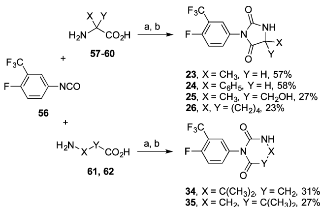
Scheme 6 a
