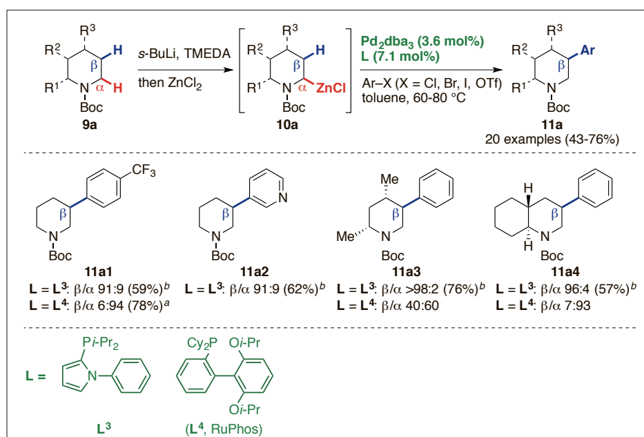
Scheme 5. \beta -Arylation of Boc-piperidines. a Yield of the isolated mixture of \alpha and \beta isomers. b Yield of the isolated \beta isomer.
