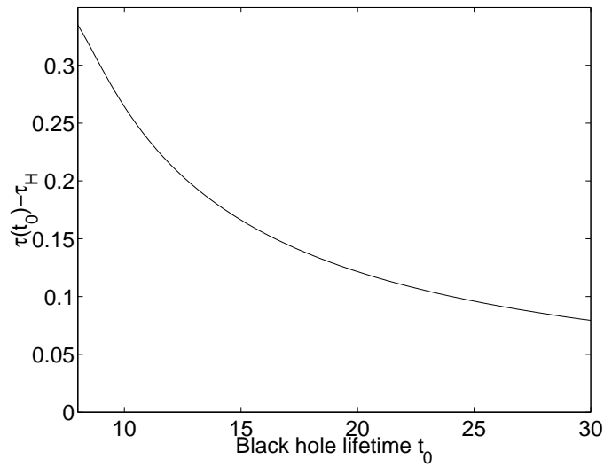
Figure 3: Eigentime \tau(t_0) reduced by the eigentime \tau_H needed by a test particle to reach the horizon of a stable black hole, versus the black hole lifetime t_0 .
