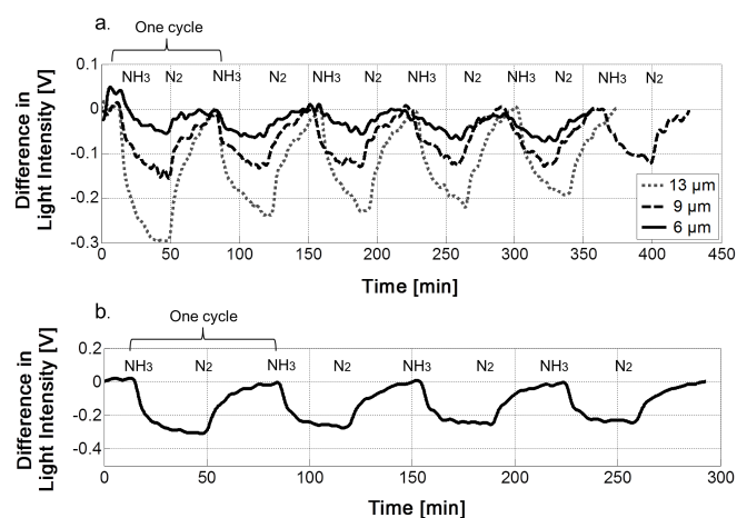
Fig. 11 a.: response and reversibility of the most sensitive (sol composed of 25 \mu\text{mol} coumarin and 6.25 \mu\text{mol} fluorescein) xerogel towards 100 ppm ammonia depending on xerogel thickness; b.: response and reversibility of a 6 \mu\text{m} xerogel to 1000 ppm ammonia.
