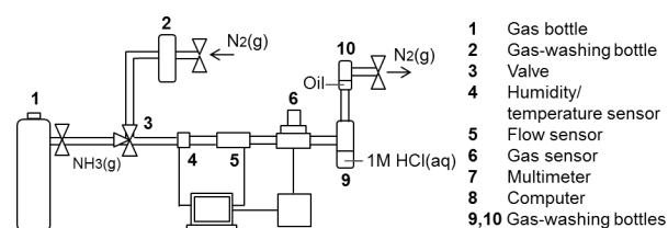
Fig. 3 Schematic of the experimental setup.
