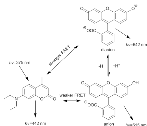
Fig. 7 Schematic of the sensing mechanism.
