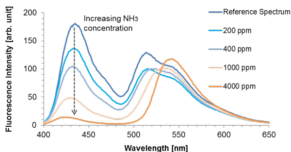
Fig. 8 Fluorescence emission spectra observed of a 1:1 coumarin:fluorescein xerogel (sol composed of 25 \mu\text{mol} coumarin and 25 \mu\text{mol} fluorescein) upon exposure to different amounts of gaseous ammonia (ex. 375 nm).
