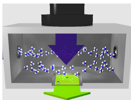
Fig. 2 Rendered impression of the flow cell showing a xerogel coated plate (shown in green) in a recessed area in the floor. The plate is illuminated from the top by a UV-LED (violet arrow) through a UV-transparent window. Fluorescence emission (green arrow) is measured through an opening in the front of the cell.
