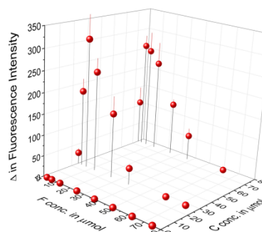
Fig. 10 3D plot illustrating the loss of fluorescence for different coumarin:fluorescein ratios upon ammonia exposure (10 3 000 ppm). The given concentrations refer to the concentrations in the starting sol solution. The samples were excited at 375 nm, and the emission measured at 442 nm.
