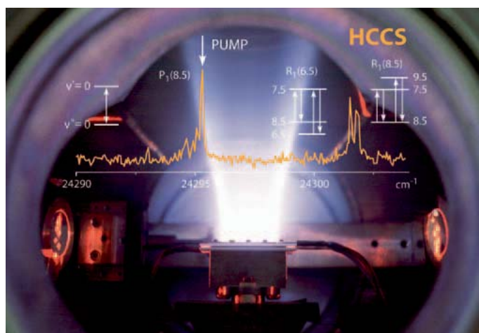
Fig. 3. Degenerate four wave mixing is a means to measure the electron spectra of transient species. The example shown is for HC_2S , produced at low temperatures in a supersonic slit jet expansion of CS_2/H_2 seeded in helium, through which a discharge runs. A two colour variant of the method is used in a double resonance mode to assign the rotational lines unambiguously.
